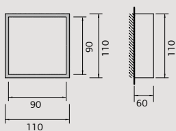
DIVETRO 9 WOOD Led 5W – 230Vac – 3000K CE Peso / Weight 0,45 kg
